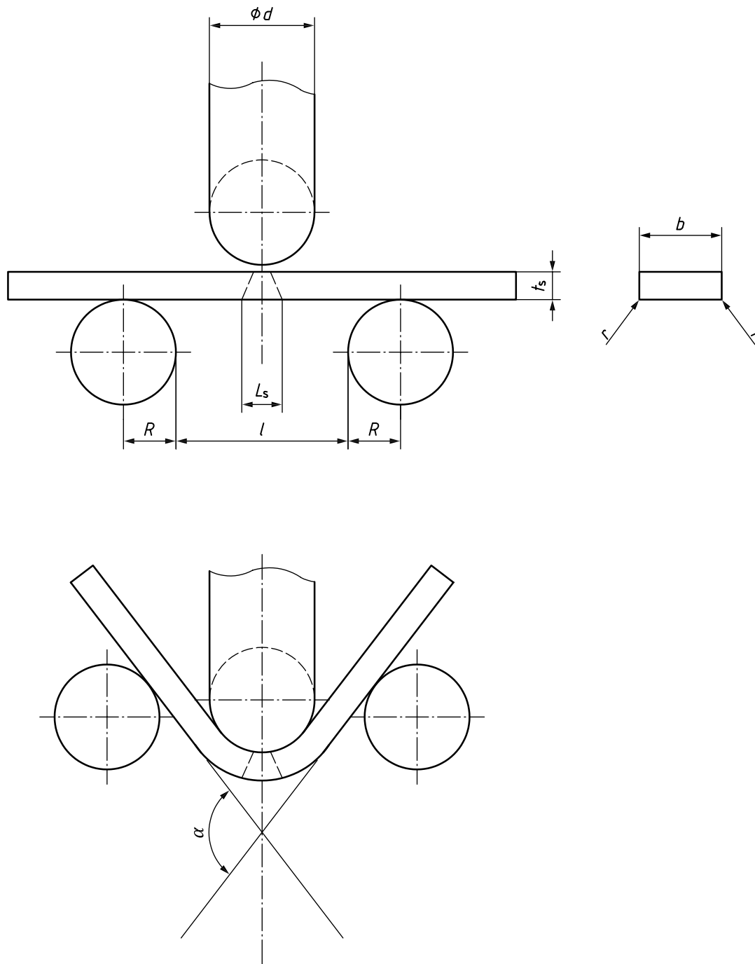
Figure 11 — Transverse face or root bend test
