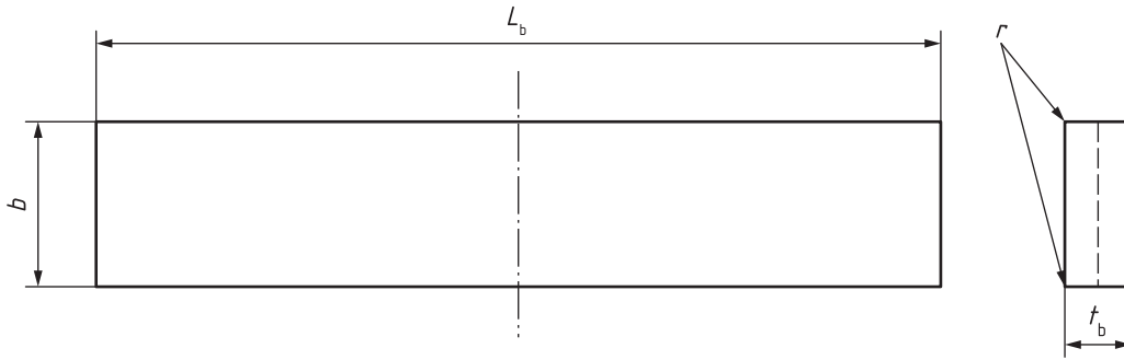
Figure 17 — Backing plate geometry
