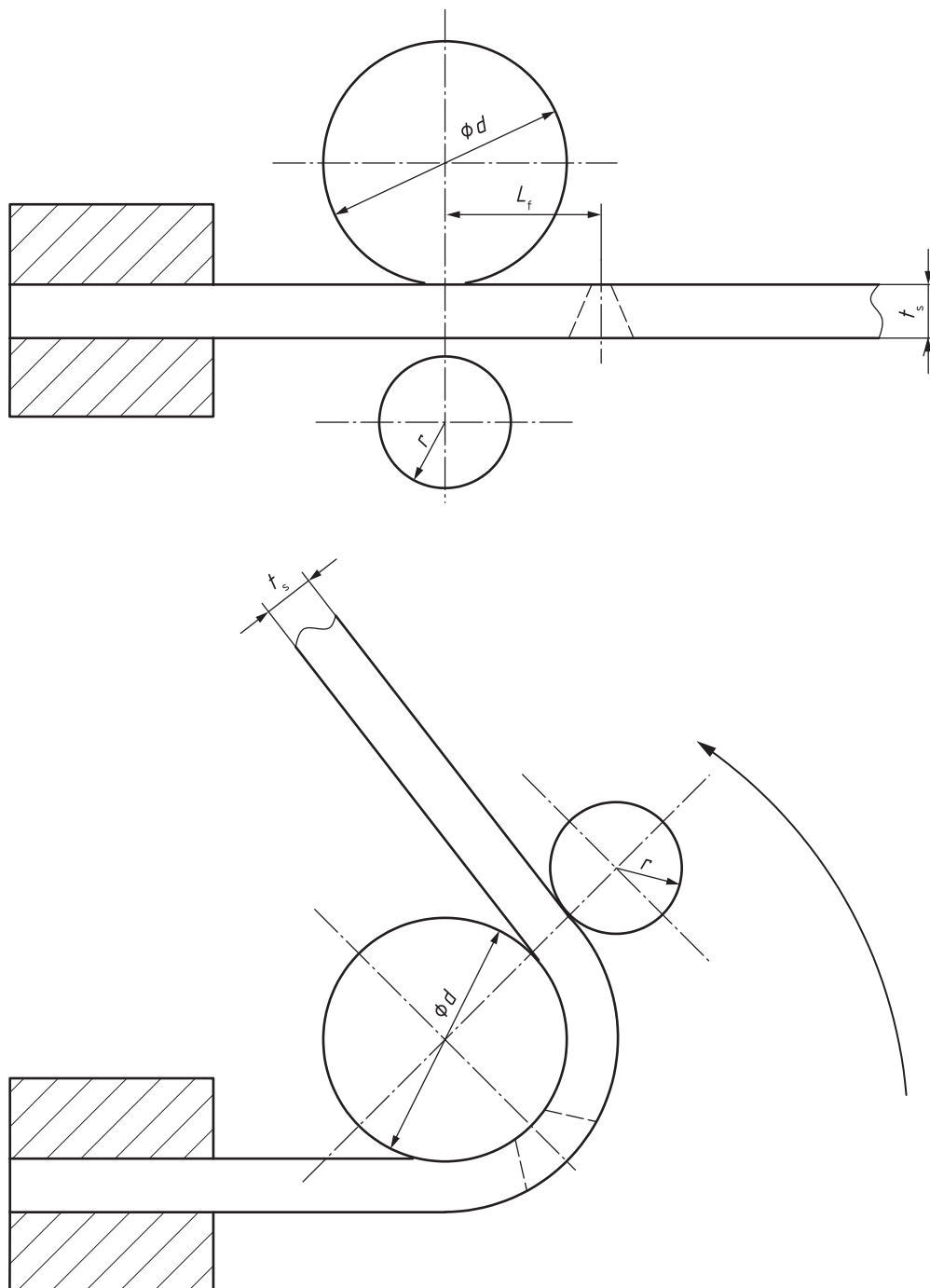
Figure 15 — Method of bend testing using a roller
