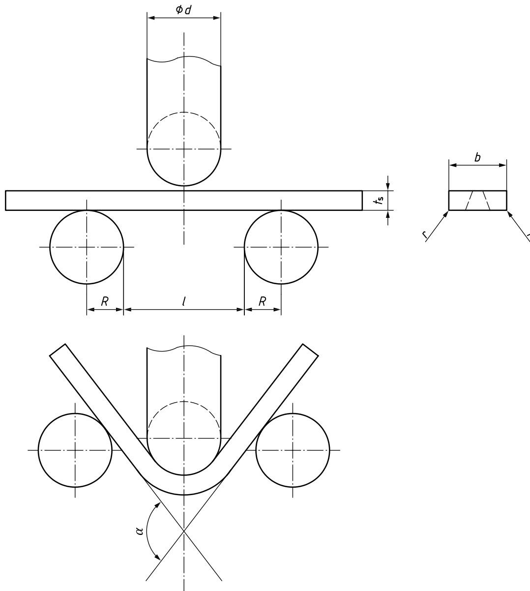
Figure 13 — Longitudinal bend test
